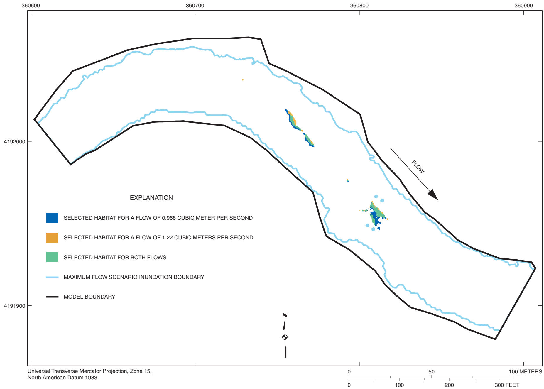
Figure 1-41. Selected habitat area distribution for habitat category 19 (stonecat) at flows of 0.968 and 1.22 cubic meters per second at Marmaton River site M1.
